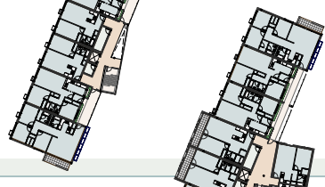
typical upper floor plan 1"=40'-0"
